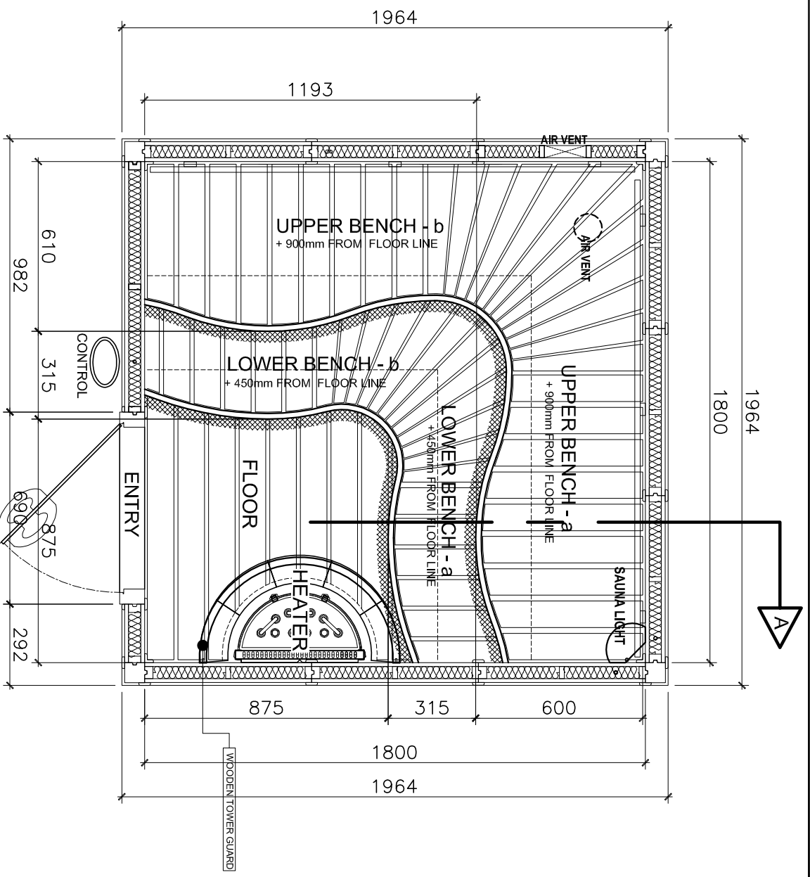
FLOOR PLAN
