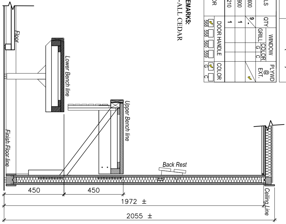
SECTION - A
