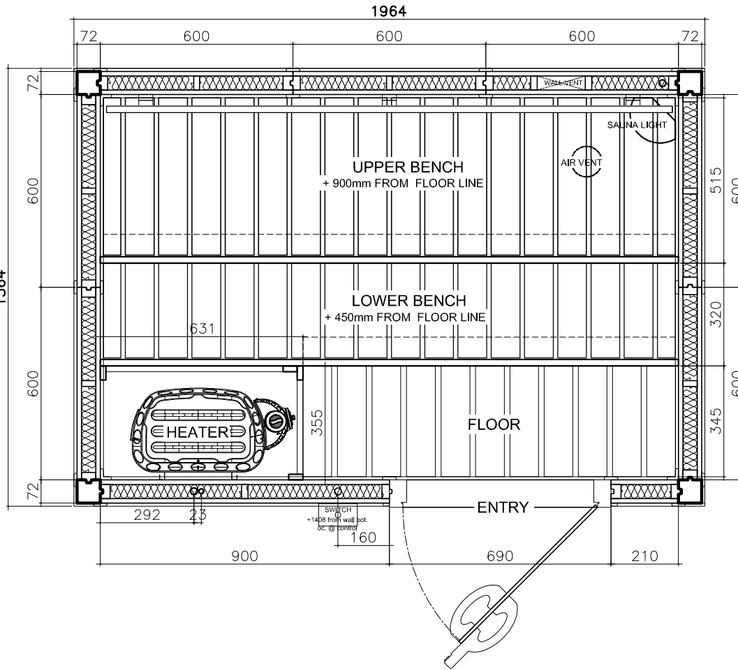
FLOOR PLAN FIT TO SCALE
