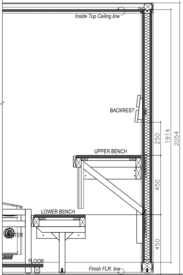
SECTION FIT TO SCALE
